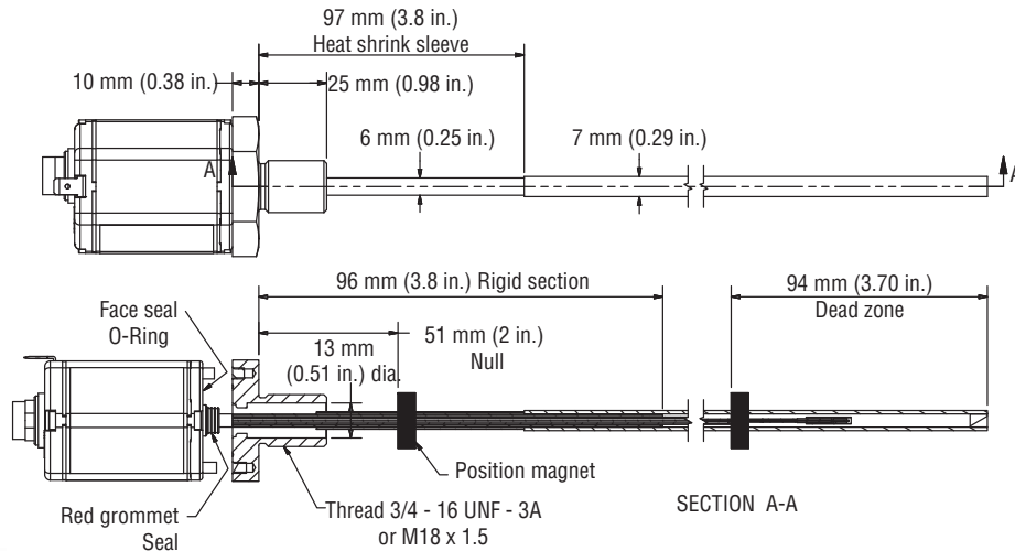
Figure 1. R-Series Model RF flexible housing dimension reference
