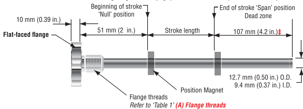
Figure 5. Style 'HL' pressure pipe (flat-faced flange shown with U.S. customary threads)
